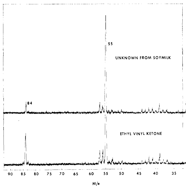
Figure 3. Mass spectra of ethyl vinyl ketone and component exhibiting green bean odor isolated from soybean milk
