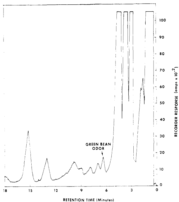
Figure 2. Gas chromatogram of components in liquid nitrogen trap
