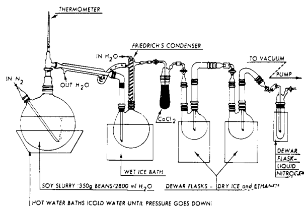
Figure 1. Distillation train for separation of green bean volatile flavor of soybeans
